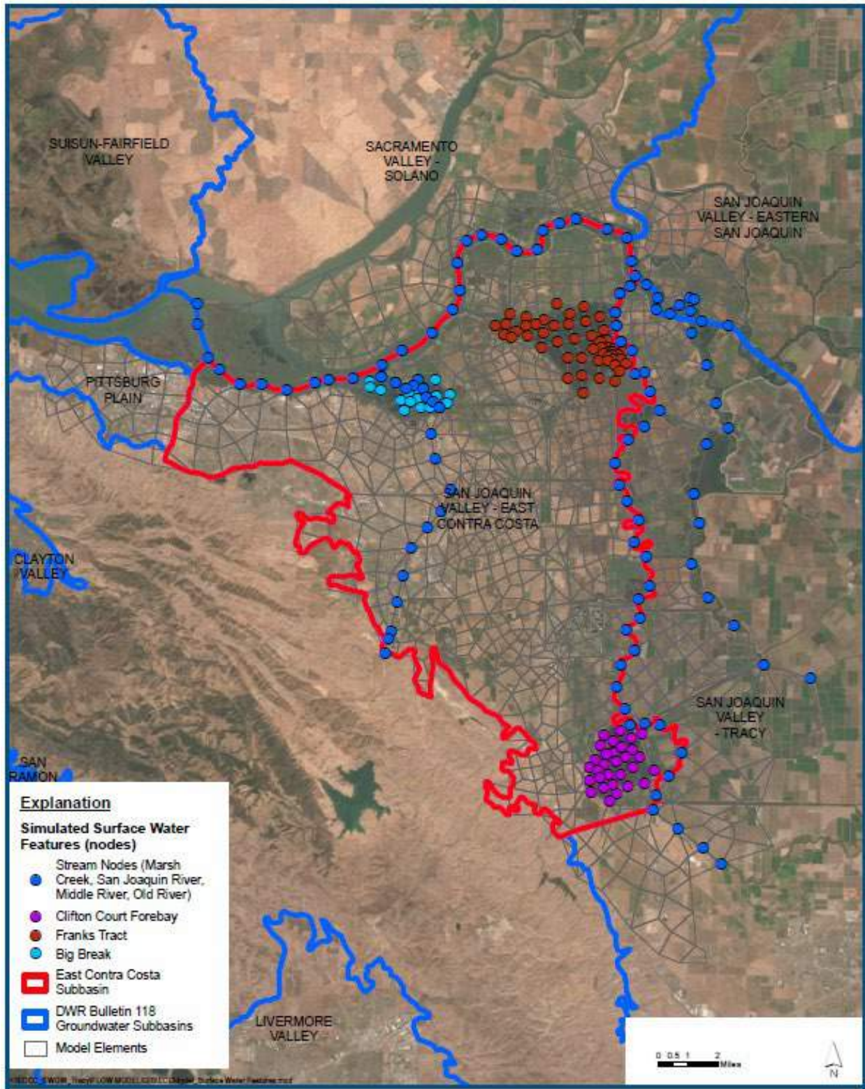
Model Nodes for Simulated Surface Water Features East Contra Costa Groundwater-Surface Water Simulation Model (ECCSim)
