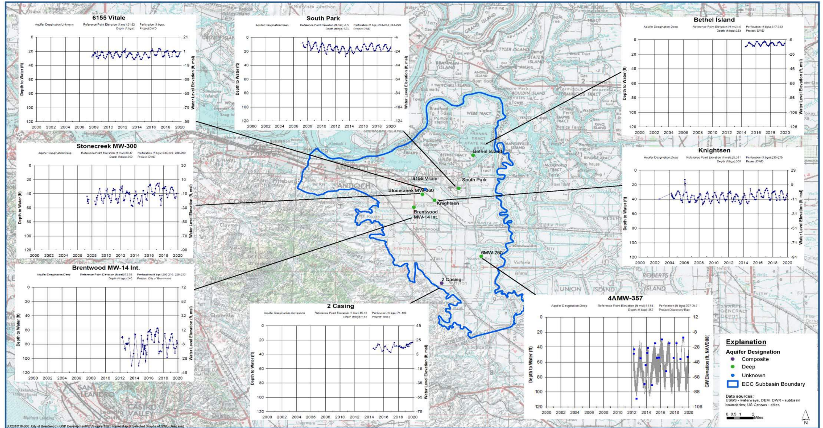
Selected Graphs of Groundwater Elevations - Deep and Composite Zone
